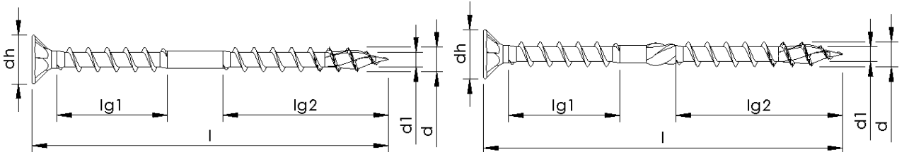
Secondary thread without variation, without shank ribs, with toothed tip and milling ribs
