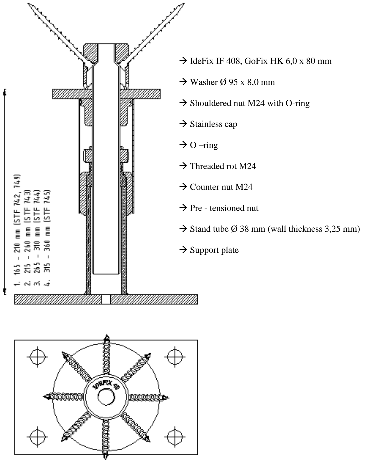
Figure 26: STF / STZ 700 series with IdeFix IF or ZaFix ZF
