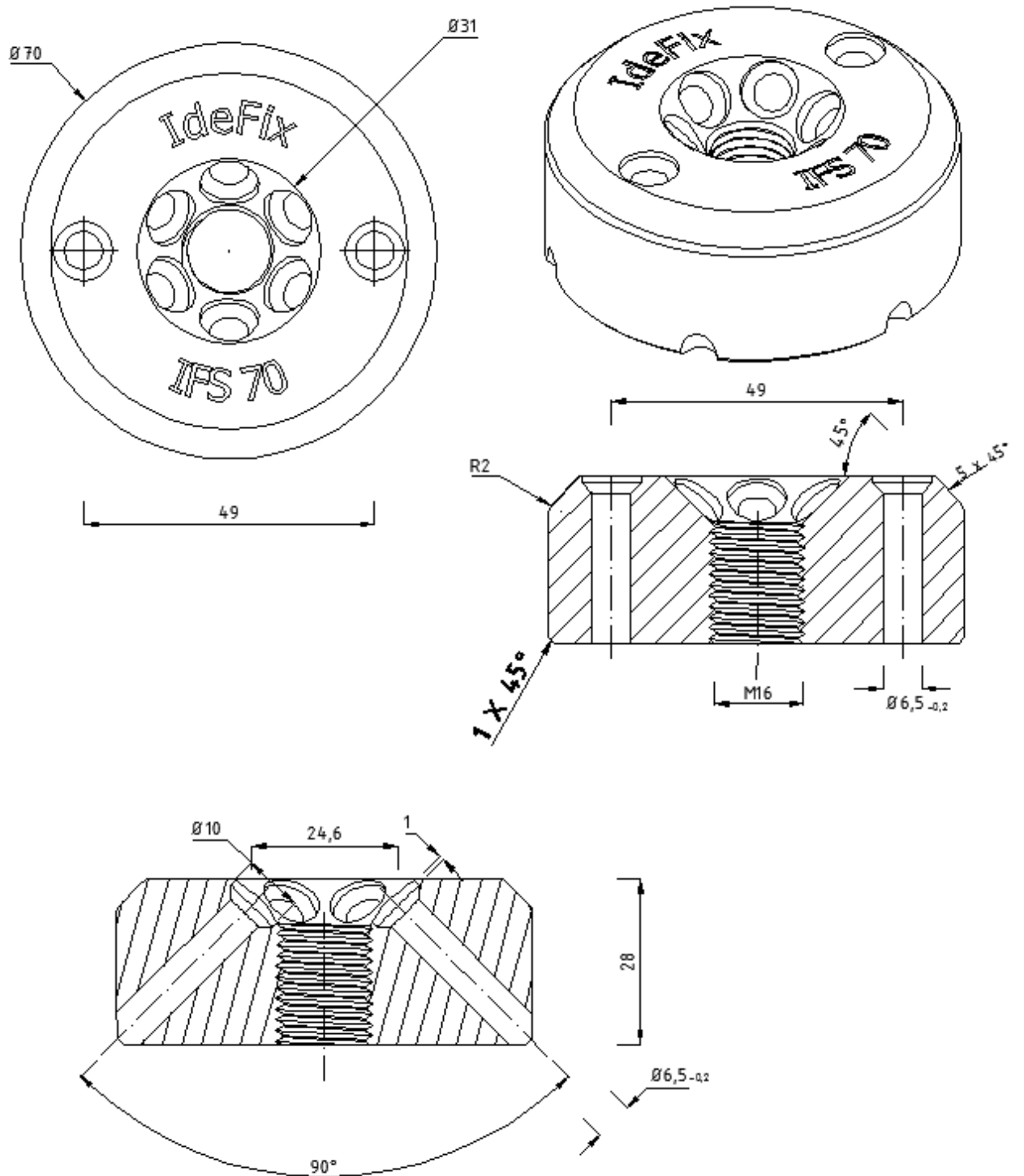
Figure 17: IdeFix IFS, details
