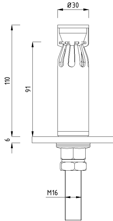
Figure 21: ZaFix ZF d=30, details
