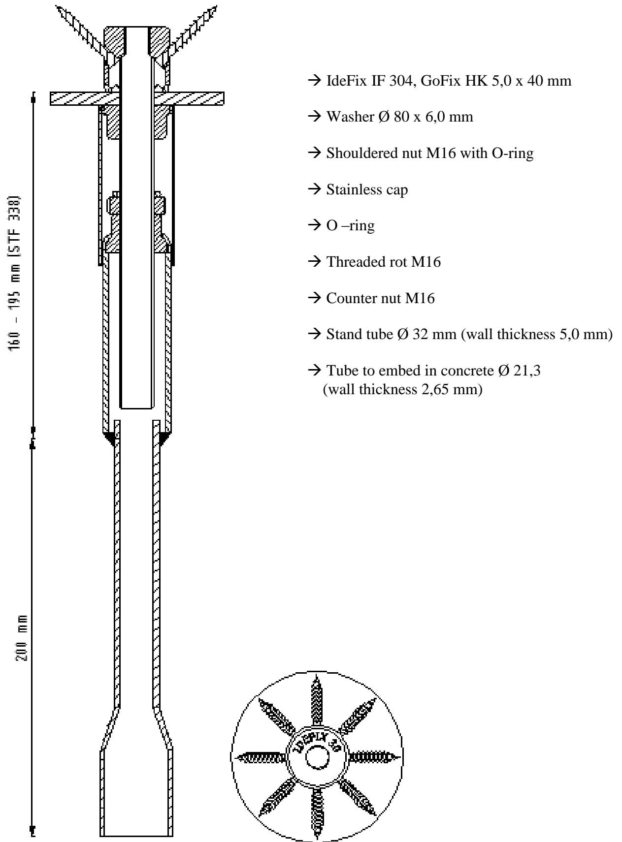
Figure 28: STF /STZ 338 with IdeFix IF or ZaFix ZF
