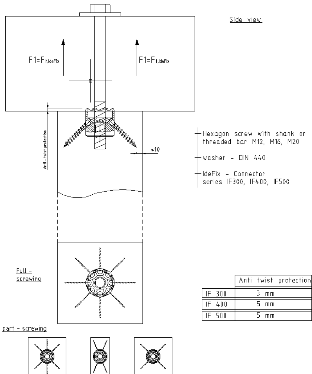
Figure 9: Tension Connection, details
