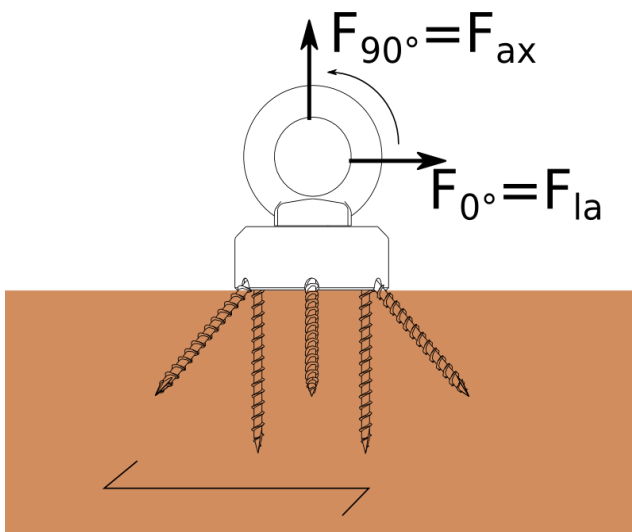
Figure 18: IdeFix IFS loading
