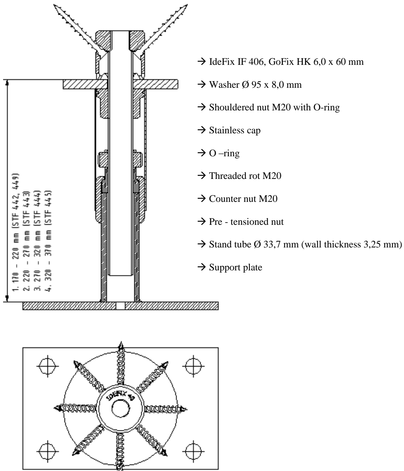
Figure 25: STF / STZ 400 series with IdeFix IF or ZaFix ZF
